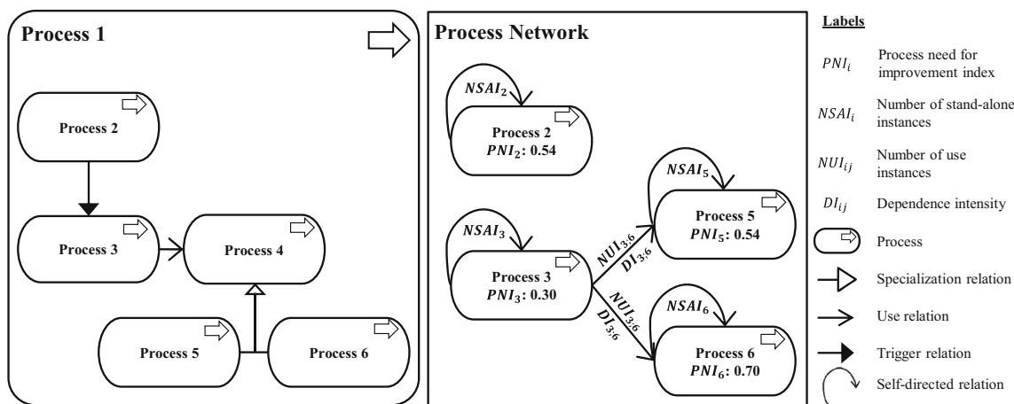
Fig. 1 Example of a BPA (left) and the corresponding process network (right)
